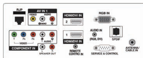
32LH200C/37LH200C/42LH200C REAR
