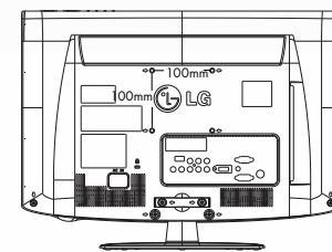
22LH200C REAR
